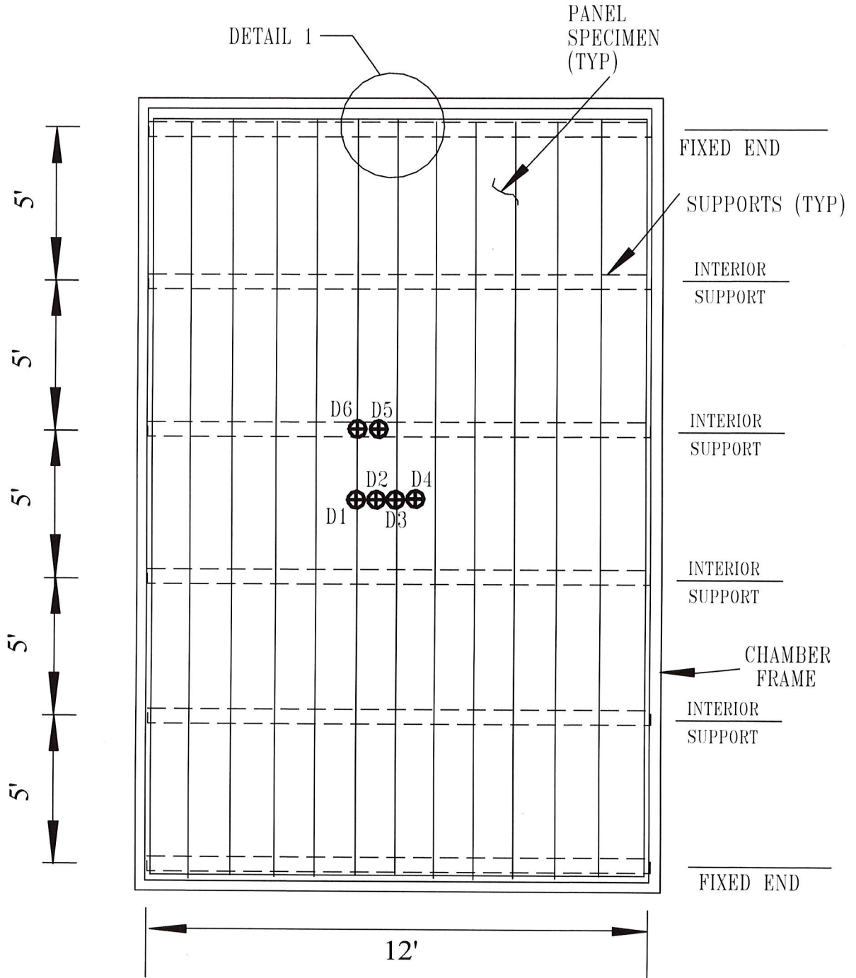
PLAN VIEW
